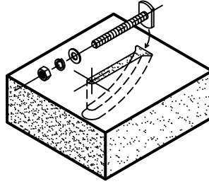
T-31 BACK ANCHOR
