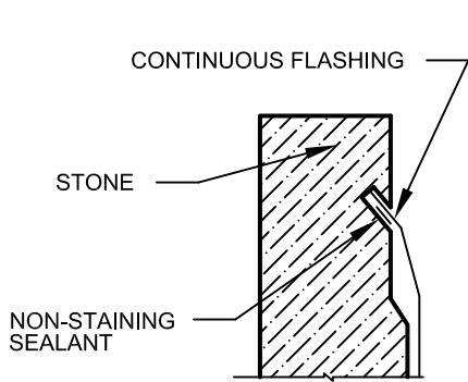
1 PARAPET DETAIL
