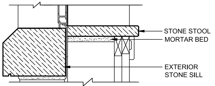
4 SECTION (MASONRY CONSTRUCTION)
