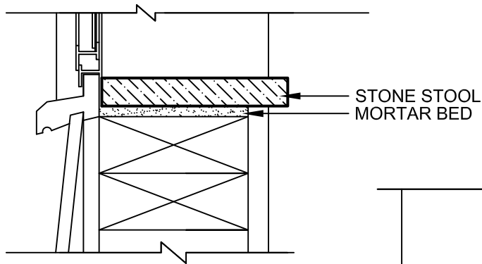
2 SECTION (WOOD FRAME CONSTRUCTION)
