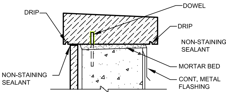
5 COPING DETAIL
