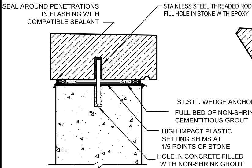
3 COPING DETAIL
