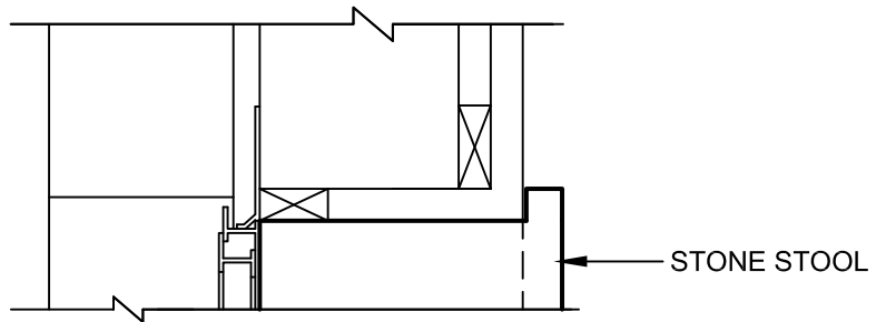
3 PLAN SECTION (MASONRY CONSTRUCTION)
