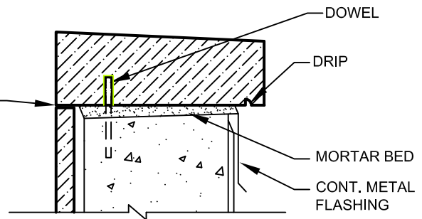
6 COPING DETAIL
