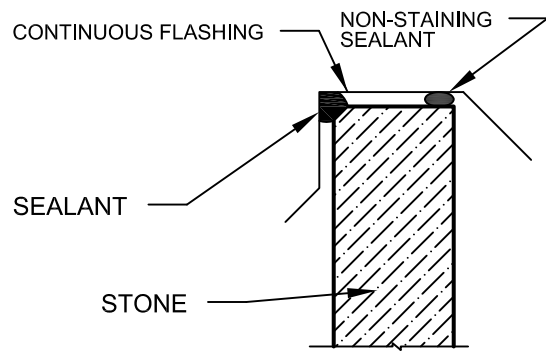
2 PARAPET DETAIL
