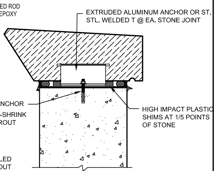
4 COPING DETAIL
