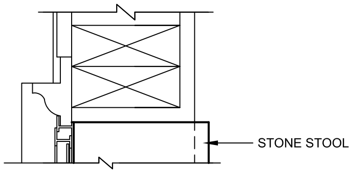
1 PLAN SECTION (WOOD FRAME CONSTRUCTION)
