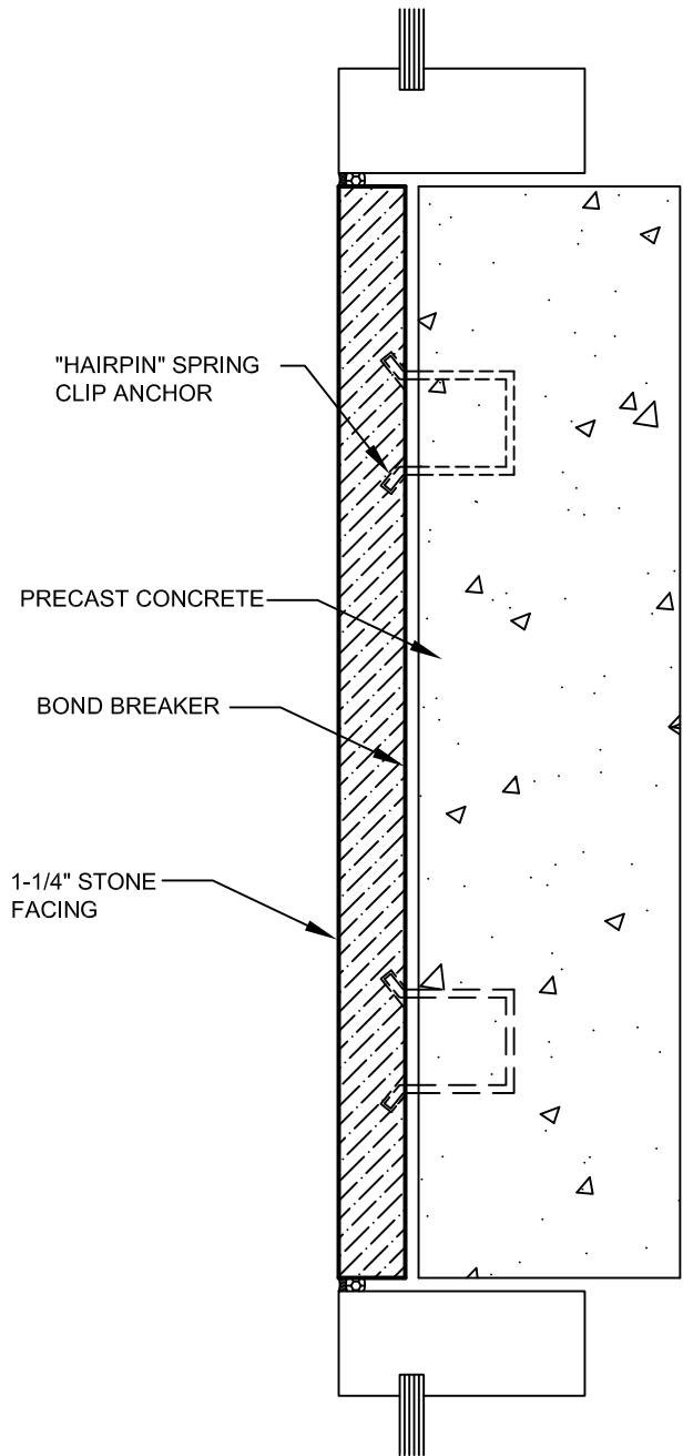
1 TYPICAL SECTION
