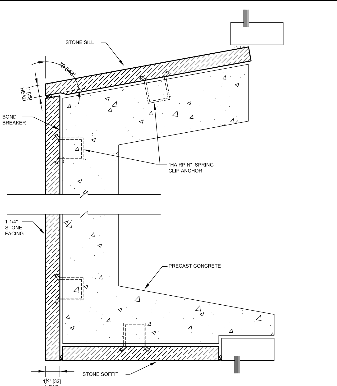
1 TYPICAL SECTION OF UNITIZED SILL, FACIA, AND SOFFIT
